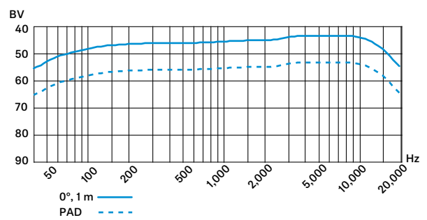
Superniere / super-cardioid
