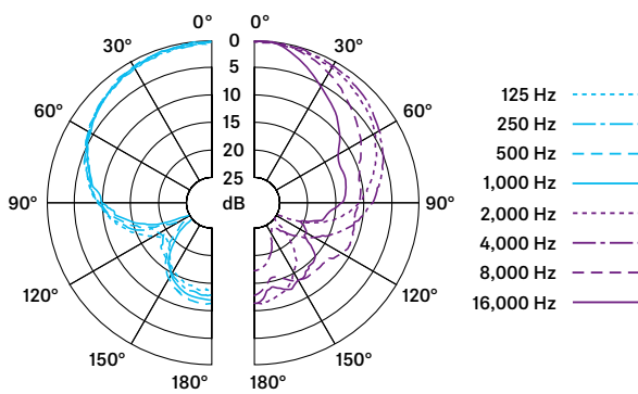
Superniere / super-cardioid
