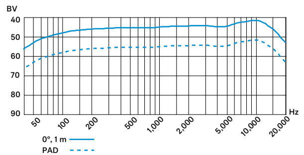
Niere / cardioid
