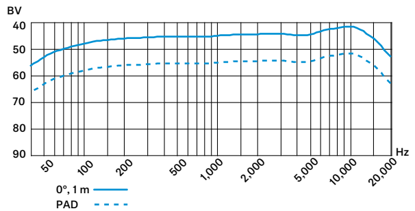
Niere / cardioid
