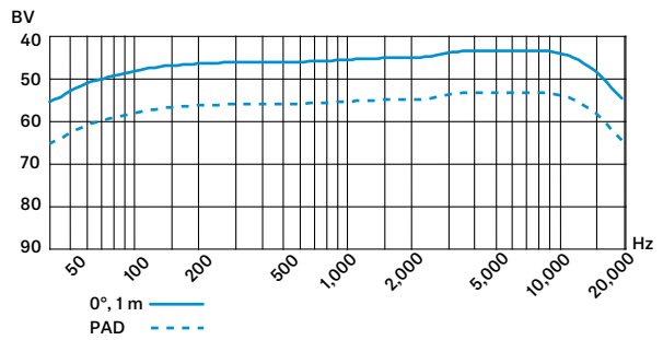
Superniere / super-cardioid
